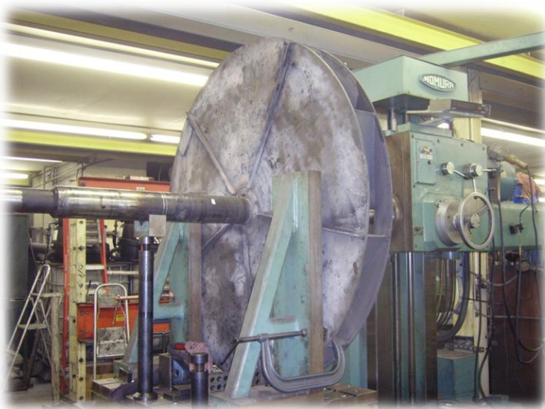
72" Diameter Fan Blade Machined in Numora Horizontal Boring Mill
